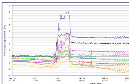
Graph showing tilt data during cold weather
